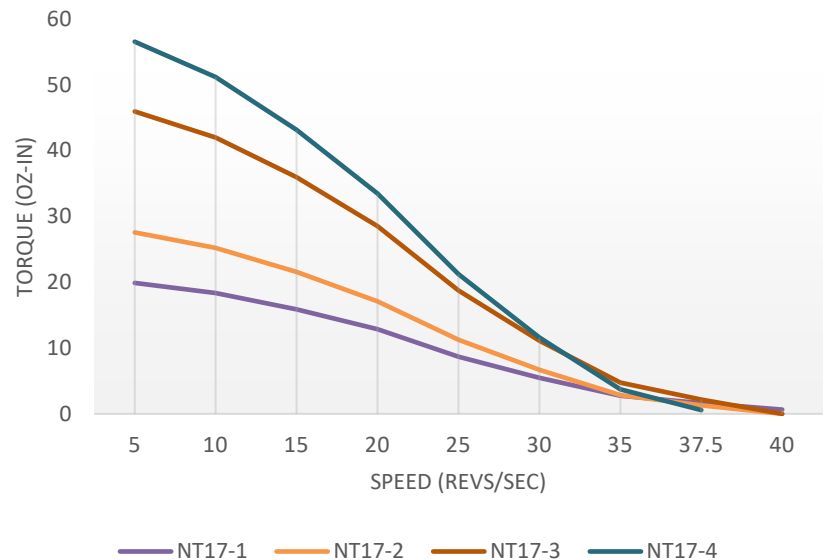
NT17 Stepper Motors (24VDC)
